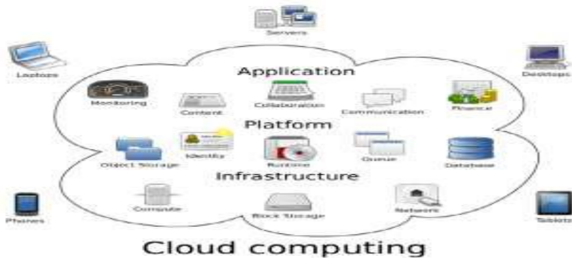
Figure 2: Cloud computing
