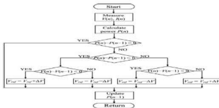
Figure 1.4: Using a P&O Algorithm
