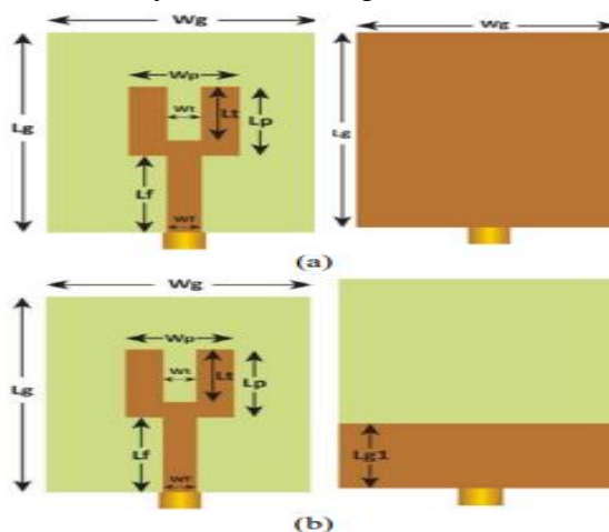
Fig 1. Antenna's Layout (A) TFS (B) PG-TFS
