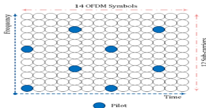
Figure 1:- An example of the time-frequency resource grid for LTE-A
