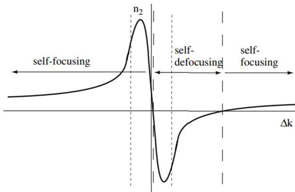
Fig. 2 The total effective n_2 resulting from both quadratic and cubic contributions plotted versus \Delta k for the typical case when X^{(3)} phase shifts are positive. Self-focusing and selfdefocusing regions are indicated. The short-dashed lines represent a possible location of the stationary boundaries.
