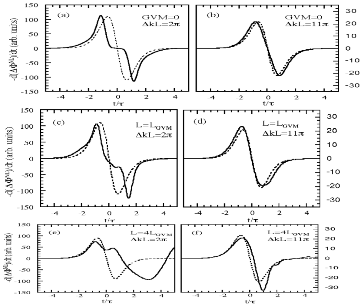
Fig. 5 Instantaneous frequency shifts of the fundamental pulse resulting from the cascaded quadratic process with the indicated values of GVM and phase mismatch. The
