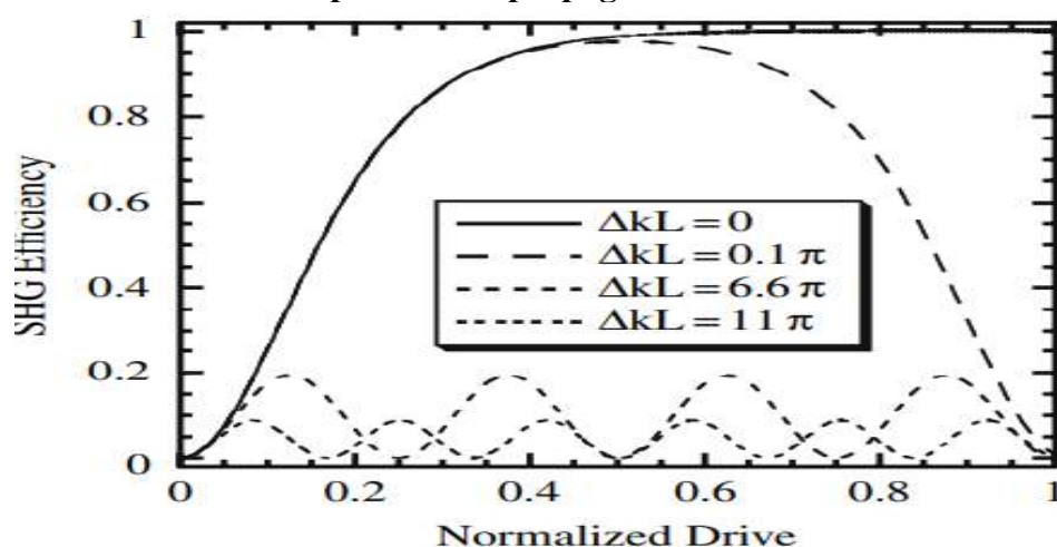
Fig. 4 SHG efficiency plotted versus nonlinear drive, which can be taken as proportional to propagation distance, for the indicated values of the phase mismatch. With larger mismatch, the conversion cycles have a smaller period, and less energy resided in the SH field
