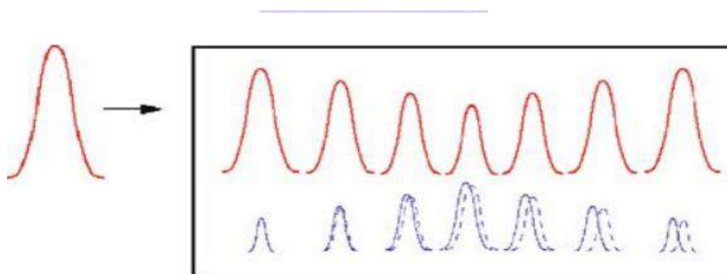
Fig. 3 Illustration of FF and SH pulses propagating in a quadratic nonlinear crystal. The dashed lines represent the propagation in the absence of GVM
